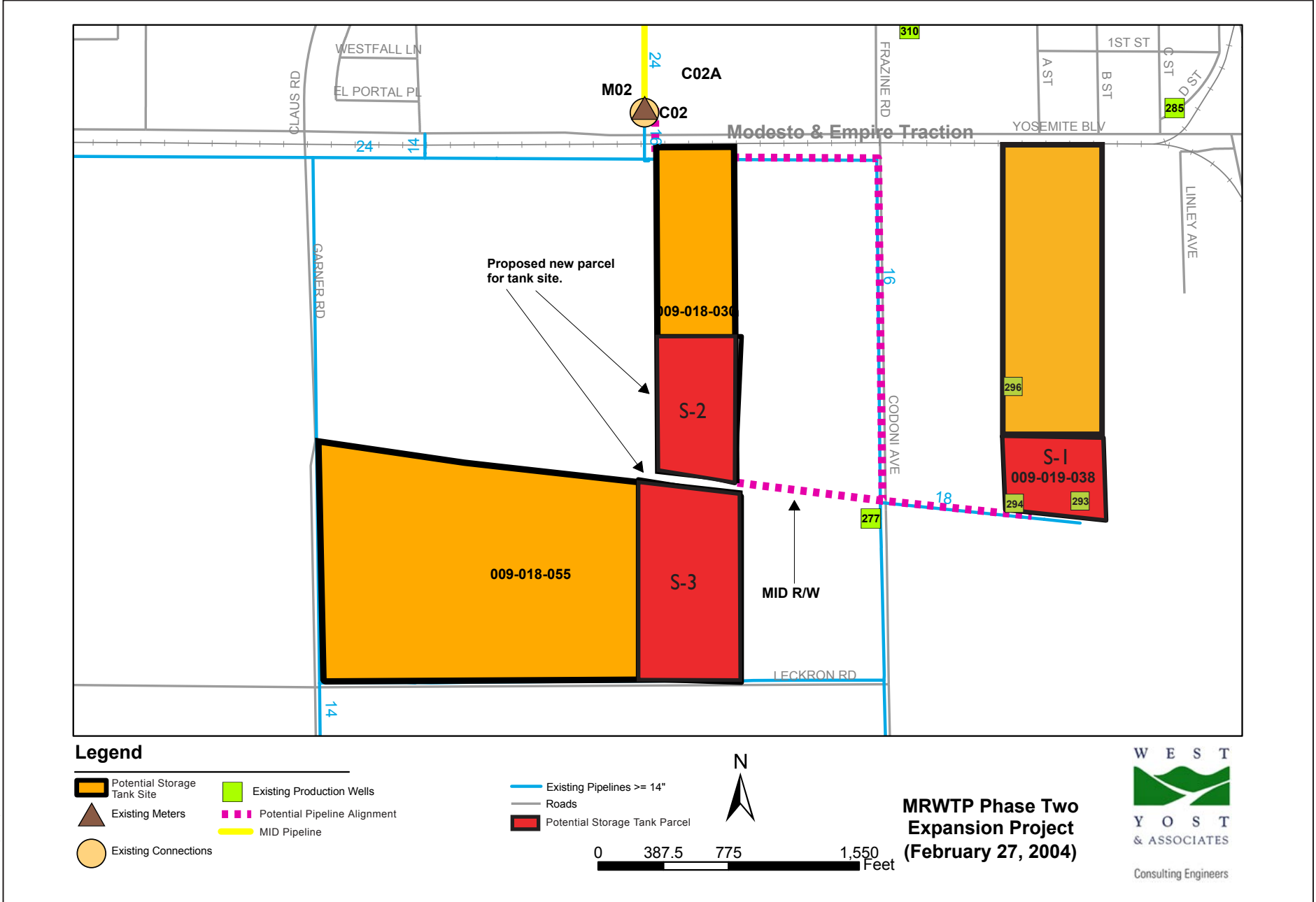
Figure 2-7 Southeast Storage Tank
