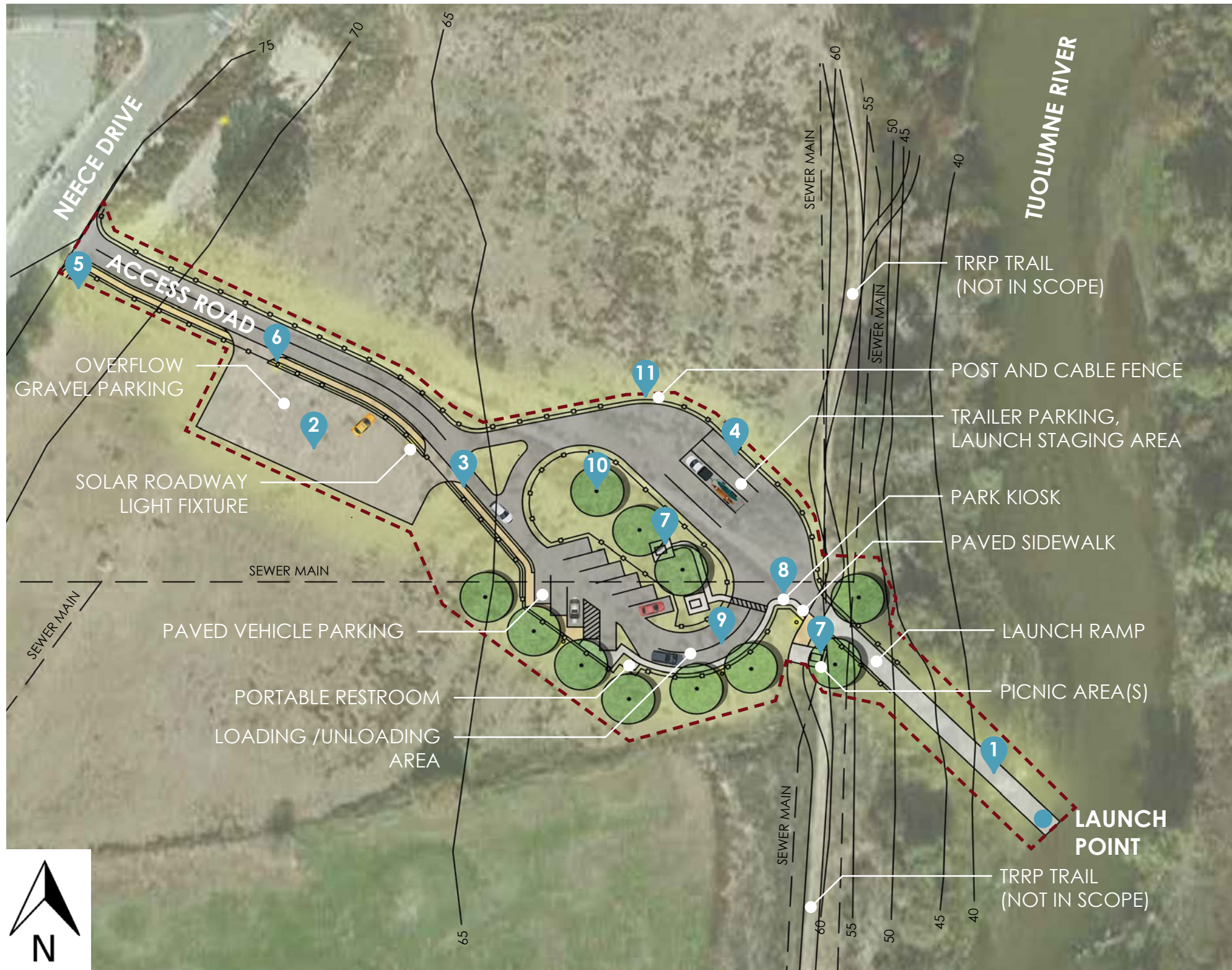
SITE PLAN, UTILITY LOCATIONS
